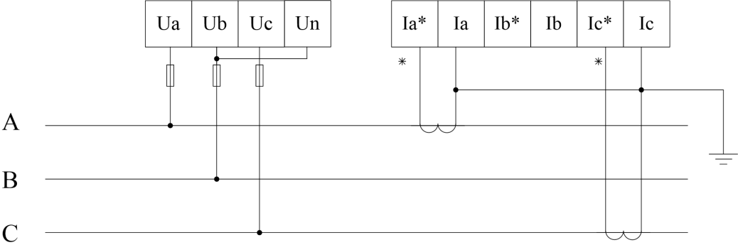
Fig 5 Three phase three lines connect via CT
