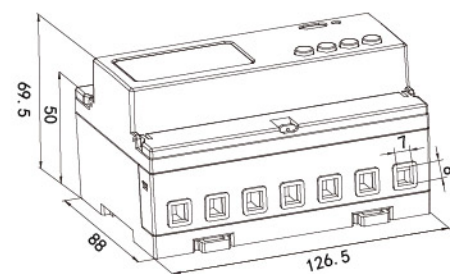
Direct connect
